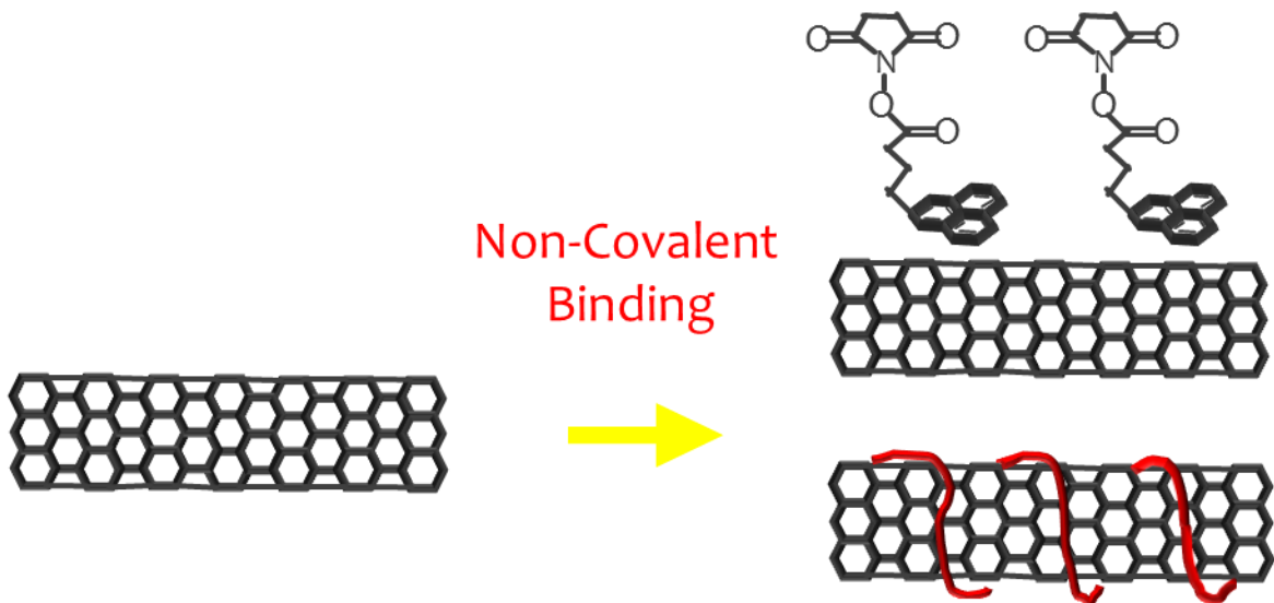
Figure 1.3. Schematic of non-covalent binding of CNTs. Upper panel on the right showed aromatic rings of adduct molecules adhere to the main body of CNTs due to \pi - \pi stacking. Bottom panel on the right showed molecular chains adhere to main body of CNTs due to van der Waals interaction and hydrophobic interactions.
